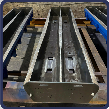
TWIN MOULD RAILWAY CONCRETE SLEEPERS
