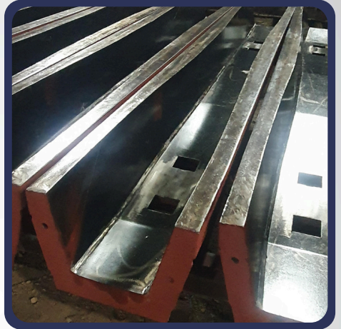
SINGLE MOULD RAILWAY CONCRETE SLEEPERS
